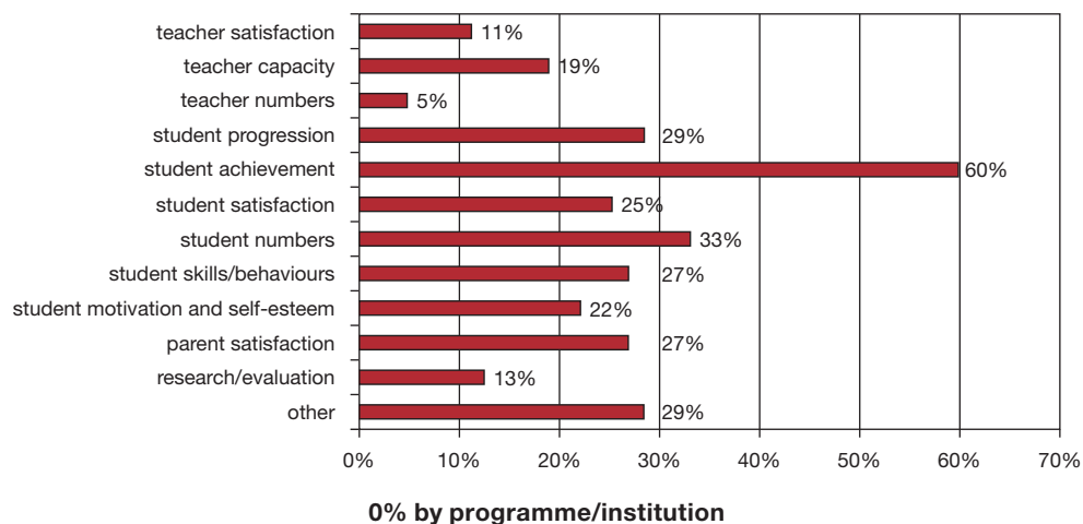
Figure 3: Success criteria
